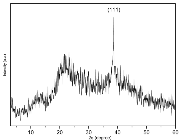
Fig. 4 XRD spectrum of PESAM/Ag nano hybrid.
