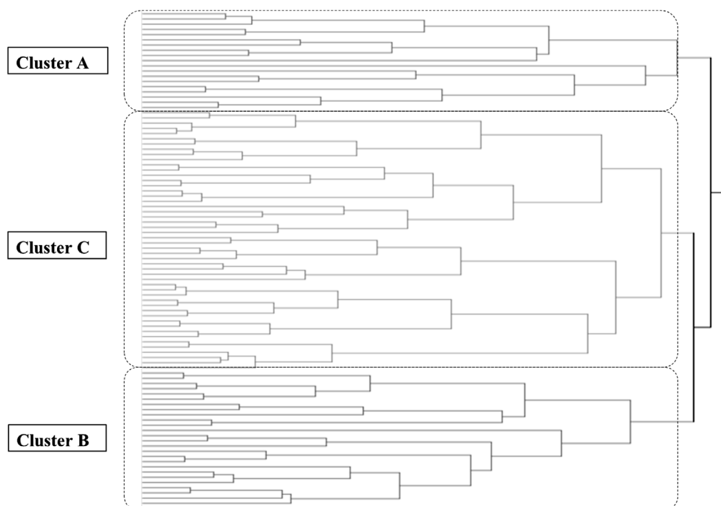
Figure 2. Cluster dendrogram. After excluding patients with missing values, 95 patients were categorized into 3 clusters.
