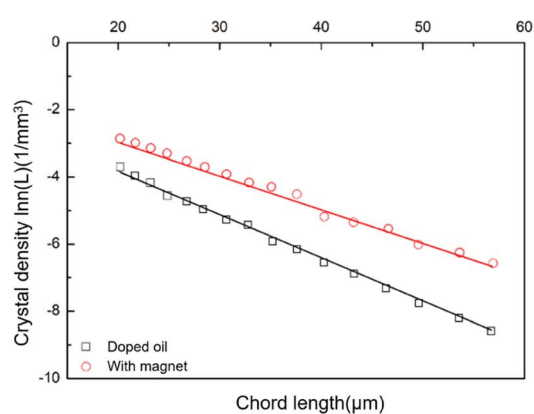
(b) Size distribution of wax crystals in the doped waxy oil before and after magnetic treatment
