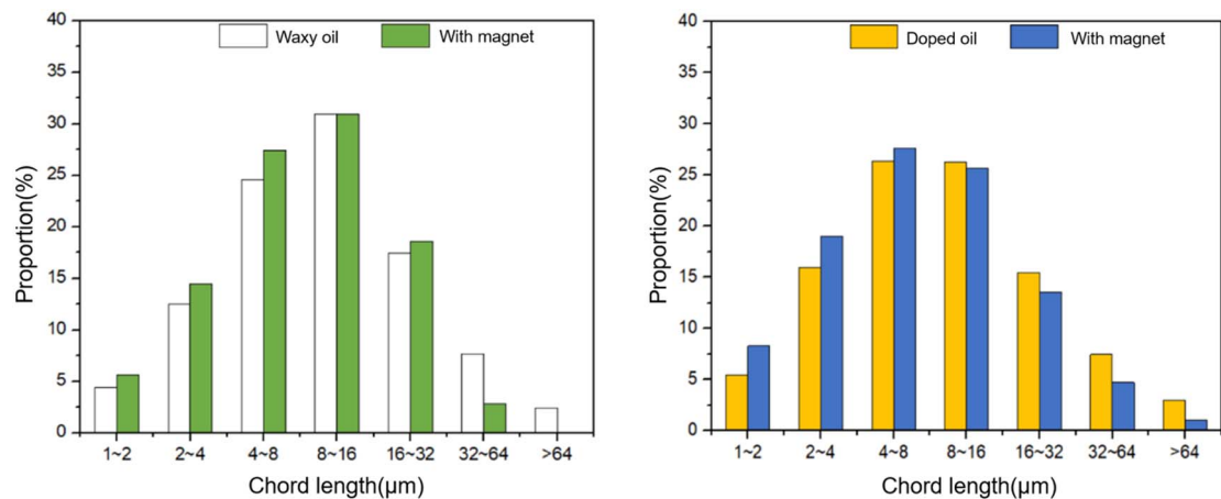
(a) Size distribution of wax crystals in the undoped waxy oil before and after magnetic treatment
