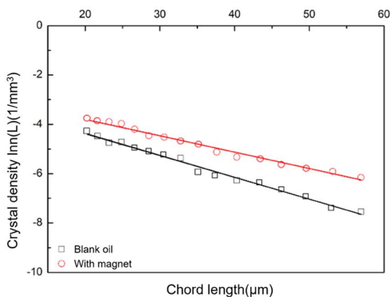
(c) SIG model fitting diagram for the undoped waxy oil before and after magnetic treatment
