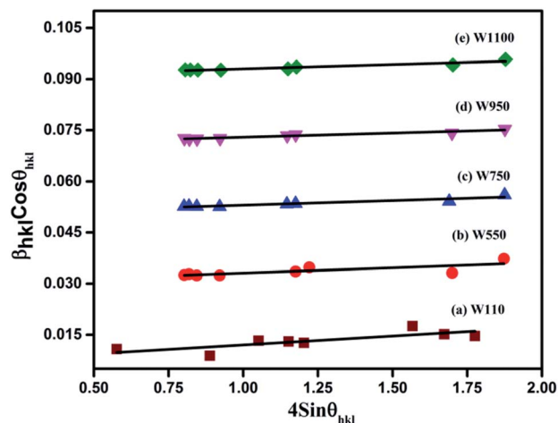
Fig. 3 The W–H analysis of the prepared samples assuming UDM. Fit to the data, the strain is extracted from the slope and the crystalline size is extracted from the y -intercept of the fit.
