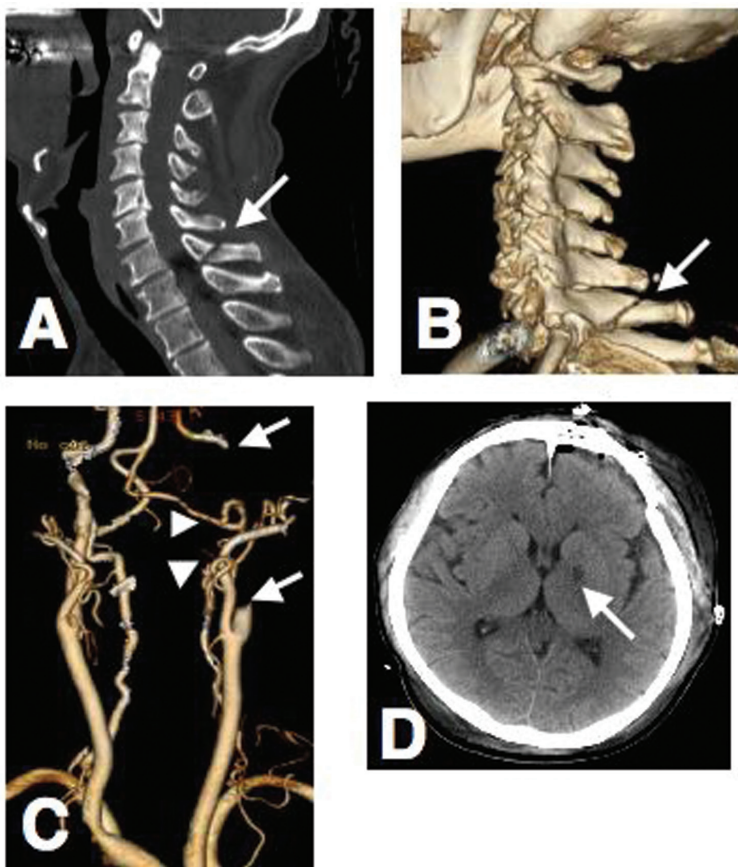
Fig. 2 Several imaging studies in a 62-year-old male (case 2). A, B: Cervical spinal computed tomography (CT) sagittal scan (A) and three dimensional (3D)-CT (B) showing spinous process fracture of 7th cervical spine ( arrow ). C: 3D-CT angiogram demonstrating an abrupt discontinuance of left Internal carotid artery ( arrows ) and vertebral artery ( arrowheads ). D: Brain CT axial scan obtained after urgent craniotomy and epidural hematoma evacuation demonstrating a cerebral infarction in the left basal ganglia ( arrow ).
