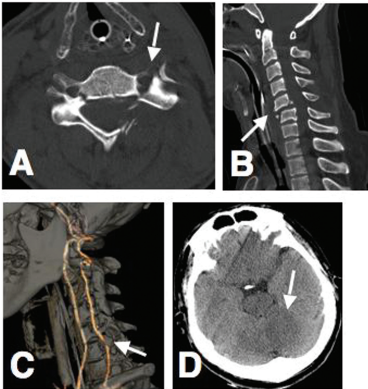
Fig. 1 Several imaging studies in a 41-year-old male (case 8). A: Cervical spinal computed tomography (CT) axial scan showing significant facet fractures extending into the foramen transversarium ( arrow ). B: Cervical spinal CT sagittal scan showing a significant subluxation at the level of C5/6 ( arrow ). C: Three dimensional (3D)-CT angiogram demonstrating an abrupt discontinuance of left vertebral artery ( arrow ) at the site of the fracture. D: Brain CT axial scan demonstrating a cerebral infarction in left cerebellar hemisphere ( arrow ).
