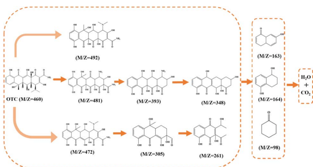
Fig. 8 Proposed OTC degradation pathways over the HCN-500/PDS system.
