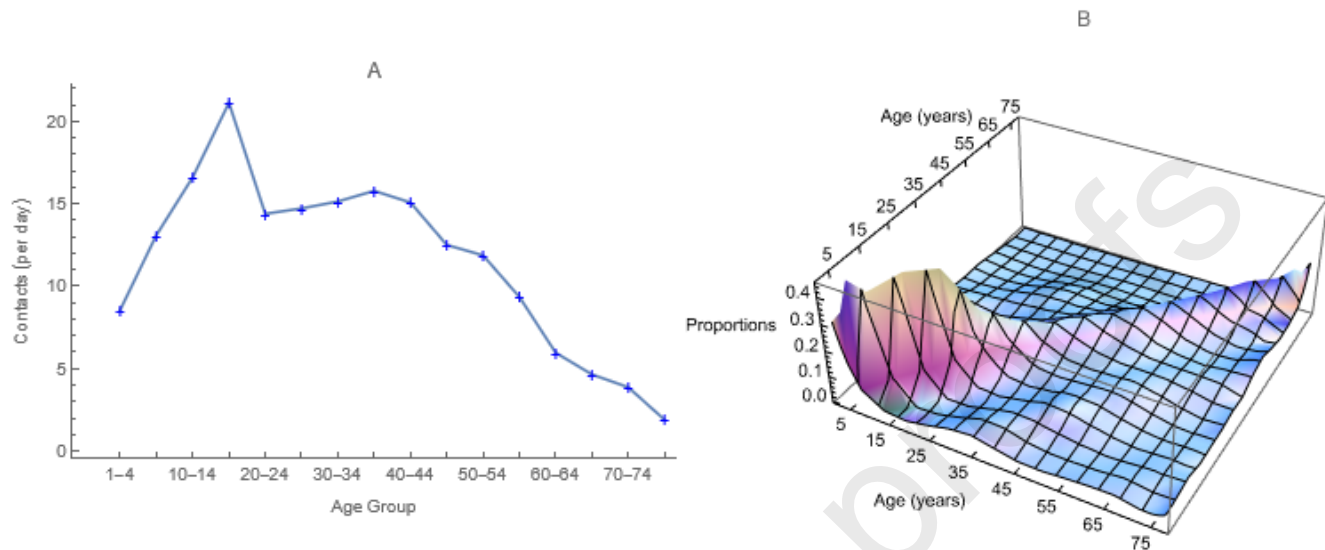
Figure 3. Parameters Derived from Synthetic US Contacts. We use these a) average marginal contact rates by age group, a_i , to which authors commonly refer as activities, and b) proportions of the contacts that members of each age group have with members of all age groups, including their own, c_{ij} .
