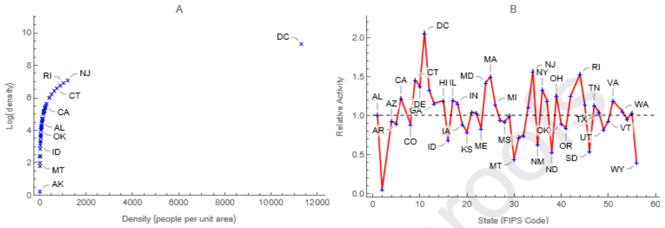
Figure 5. Contacts are a Function of Population Density. Multiplying contacts within locations (figure 3a) by ratios of natural logs of population density, a) saturating functions of density, and that of the entire country, b) reduces to twofold the difference in activities between the most and least densely populated locations.
