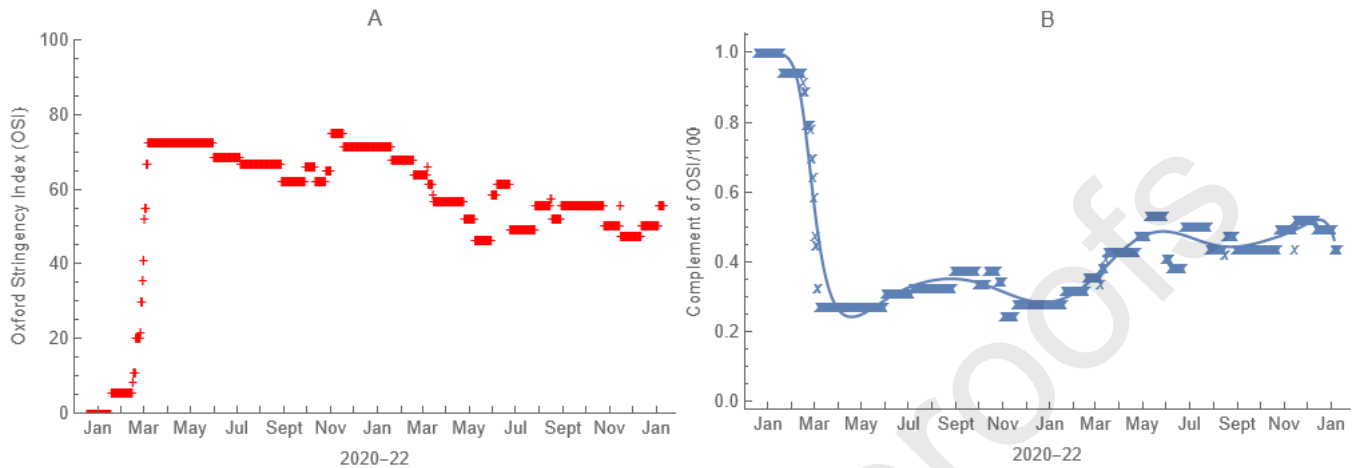
Figure 7. Effect of Non-pharmaceutical Interventions. From a) time-varying Oxford Stringency Indices for each location, illustrated here for the entire United States, we derive b) functions by which we multiply age-specific contact rates to account for local governmental efforts to mitigate the pandemic.
