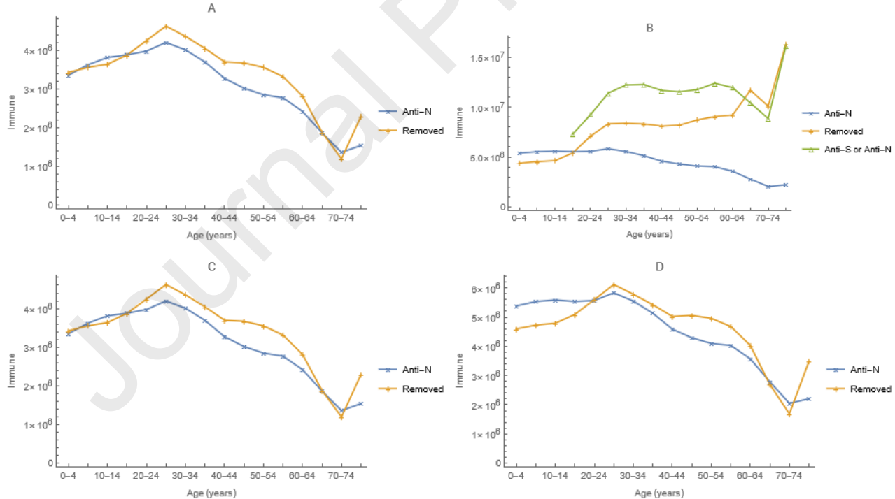
Figure 8. Observed numbers with antibodies to SARS-CoV-2, from the national commercial laboratory (Anti-N) or blood donor (Anti-S or Anti-N) seroprevalence study, and predicted numbers temporarily immune (Removed) from simulations with (A and B) and without (C and D) vaccination on 25 December 2020 (A and C) and 4 April 2021 (B and D). Vaccination had no discernible impact on 25 December 2020 serology.
