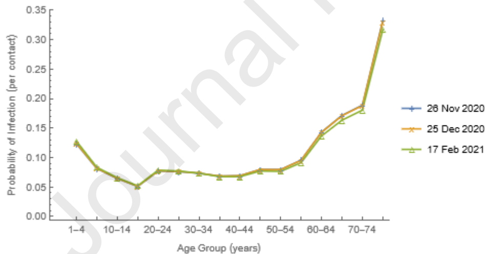
Figure 4. Probabilities of Infection upon Contact. We estimated other parameters of the n equations, \lambda_i = a_i \beta_i \sum_{k=1}^n c_{ik} (I_k / N_k) , from the information illustrated in figure 2a and synthetic US contact matrix (figure 3) and then solved them simultaneously for these unknown probabilities, \beta_i .
