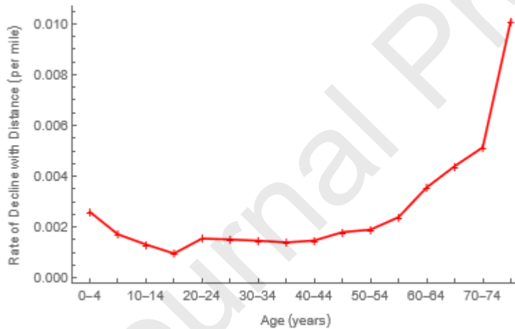
Figure 6. Rates at which Contacts Decline with Distance. Proximity to others affects the probability of contacting them. Feng, et al. (2017) assumed an exponential function. Distances are between population centers ( https://www.census.gov/geographies/reference-files/2010/geo/2010-centers-population.html ).
