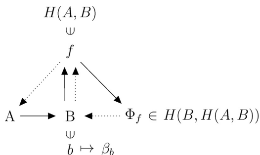
Fig. 1. Closure to efficient causation: This diagram (adopted from Rosen (1991, chapter 10)) illustrates the different processes that the individual components of the (M, R) system in (3) are involved in. On the one hand, solid arrows show where transformations from input material to output material occur— A is transformed to B , B is, in turn used for “repairing” f whereas f is transformed in order to repair \Phi_f . On the other hand, for the broken arrows, a component located at the start of an arrow indicates the initiation of a transformation located at the arrow tip— f catalyses the “metabolic” transition of A to B , \Phi_f acts on B for repairing f and the replication map \beta_b starts the repair of \Phi_f by transforming f . It is clear that each of the components f , \Phi_f and \beta_b regulates the repair of another component. In Rosen's words, the sets A, B, H(A, B) and H(B, H(A, B)) can be regarded as “material causes” whereas f, \Phi_f and \beta_b are “efficient causes”. Because each of the components is in turn produced by one of the other components the system is closed to efficient causation.
