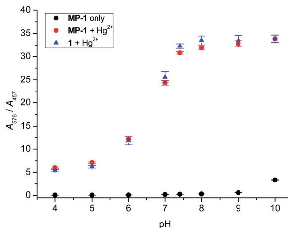
Fig. 3 Effect of pH on \text{Hg}^{2+} signaling of MP-1 expressed by changes in absorbance ratio ( A_{576}/A_{457} ). [MP-1] = [1] = 5.0 \mu M, [\text{Hg}^{2+}] = 100 \mu\text{M} , [citrate] = 5.0 mM, [PBS 7.4] = 10 mM in aqueous solution containing 20% (v/v) acetonitrile. The pH of the solution was adjusted by the addition of 1 N HCl or NaOH. Number of measurements ( n ) = 3.
