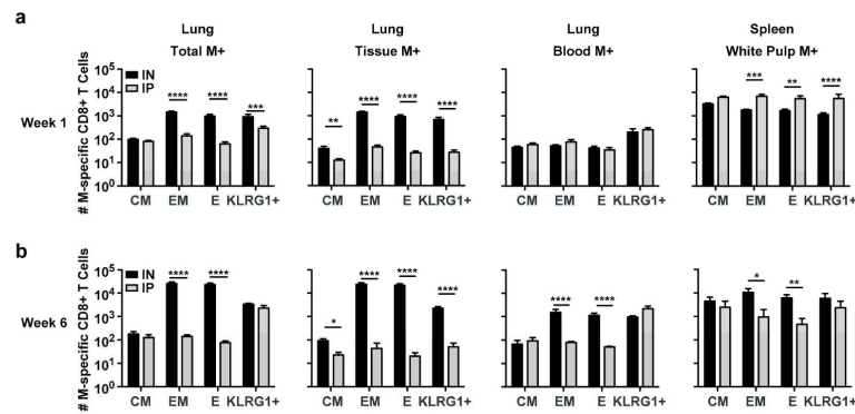
Figure 3. IN vaccination with MCMV-M augments the M-specific CD8 + T cell response via the induction of effector and effector memory cells in the lung parenchyma and blood
