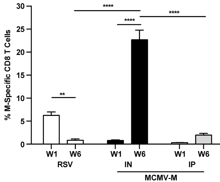
Figure 1. MCMV-M generates an M-specific CD8+ T cell population that inflates over time Mice were infected with 2 \times 10^6 PFU of RSV via the intranasal (IN) route or 6 \times 10^5 PFU of MCMV-M via the IN or intraperitoneal (IP) route. At week 1 (W1) and week 6 (W6) post-infection, the percentage of M-specific CD8+ T cells in the lungs was determined using tetramer staining and flow cytometry. Bars represent mean \pm SEM with 5 mice per group. **** p 0.0001 and **p<0.01 by two-way ANOVA with Tukey's post-test for multiple comparisons. Data represent two independent experiments.
