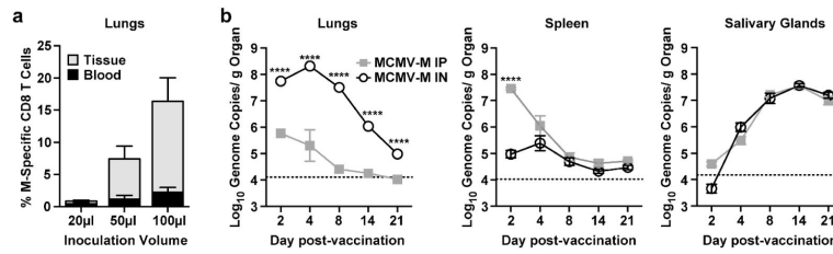
Figure 4. Large volume IN vaccination leads to increased viral replication in the lung and is necessary for the generation of tissue-tropic M-specific CD8+ T cells
