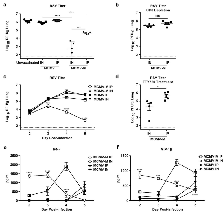
Figure 5. IN vaccination with MCMV-M leads to earlier anti-viral responses compared to IP vaccination
