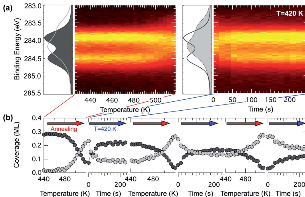
Fig. 7 (a) Left – A C 1s TP-XPS experiment performed with photon energy h\nu = 400 eV for 0.3 ML of pentacene at 0.25 \text{ K s}^{-1} , abruptly interrupted at 520 K. Right – A hydrogen uptake experiment, performed at 420 K, for the dissociated pentacene molecules. (b) Several sequential plots of the intensities of pentacene (black) and dissociated pentacene (gray) during 3 dehydrogenation/rehydrogenation cycles, the first of which is shown in (a).
