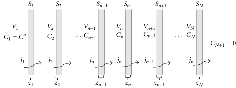
FIGURE 2: Schematization of diffusion through the multilayer thin film of the bag.
