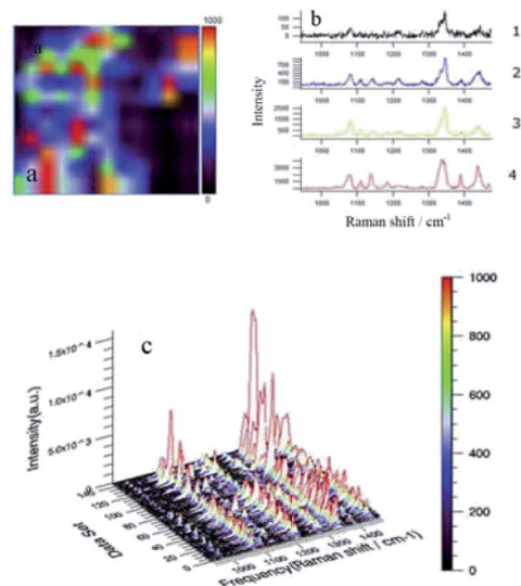
Fig. 5 Raman mapping of 5\ \mu\text{L} PNTP at a concentration of 10^{-3}\text{ M} , a wavelength of 633 nm and power of 0.5%. (a) The intensity map of all points in the sweep area based on the 1432\text{ cm}^{-1} peak; (b) the representative Raman spectra of the different color regions ((b1) black region, (b2) blue region, (b3) green area, (b4) red region); and (c) 3D distribution map of all Raman scanning points on the silver foil surface.
