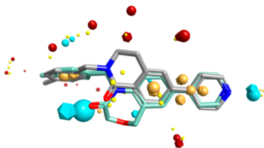
Figure 3. Overlay of 1 (OX02983) (light blue) and 28 (OX3699) (gray); blue spheres represent negative electrostatic field, red spheres represent positive electrostatic field, brown spheres represent hydrophobicity, and small yellow sphere represent the van der Waals force.
