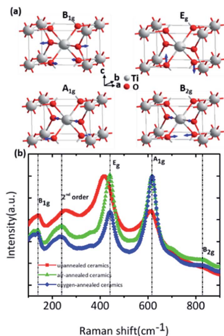
Fig. 2 (a) Raman active modes' eigenvectors of rutile \text{TiO}_2 (the sizes of eigenvectors have been enlarged to clarify the movements of atoms); (b) Raman spectra of as-prepared (Nb + In) co-doped rutile \text{TiO}_2 ceramics.
