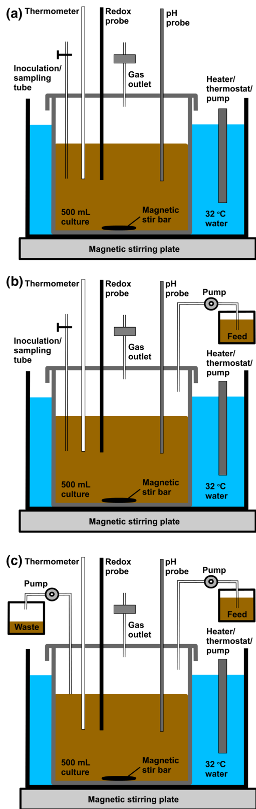
Fig. 1. Schematic diagrams of the anoxic bioreactor units. (a) Batch fermentation system. (b) Fed batch. (c) Continuous culture.
