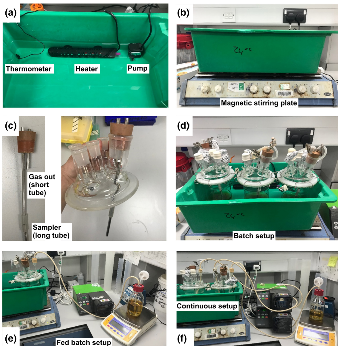
Fig. 2. Components and final setup of the anoxic bioreactor. (a) Temperature control system. (b) Mode of agitation. (c) Gas outlet and sampling tubes. (d) Three parallel bioreactors in batch mode. (e) Fed-batch mode. (f) Continuous culture mode.
