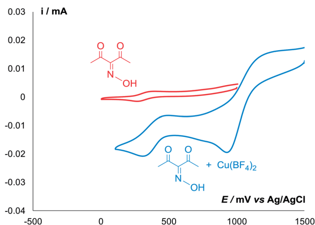
Fig. 1 CV curves of 5 \text{ mmol L}^{-1} of oxime 2a in the presence (blue) and absence (red) of equimolar amount of \text{Cu}(\text{BF}_4)_2 in 0.1 \text{ M } n\text{-Bu}_4\text{NBF}_4/\text{MeCN} at a scan rate of 0.1 \text{ V s}^{-1} at 298 K.
