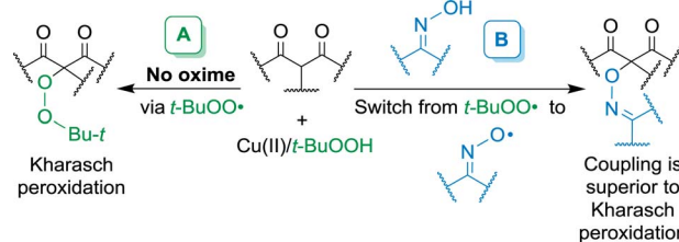
Scheme 1 Kharasch peroxidation (A) and the discovered cross-dehydrogenative C–O coupling of \beta -dicarbonyl compounds with oximes (B).
