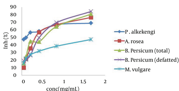
Figure 1. The Effect of Different Concentrations of P. alkekengi , A. rosea , B. persicum and M. vulgare on Mushroom Tyrosinase Activity for the Catalysis of L-Dopa
