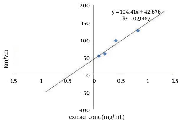
Figure 3. The Slope of Lineweaver–Burk Plots Versus the Concentration of P. alkekengi for Determination of Inhibitory Constant ( K_i ) of Tyrosinase
