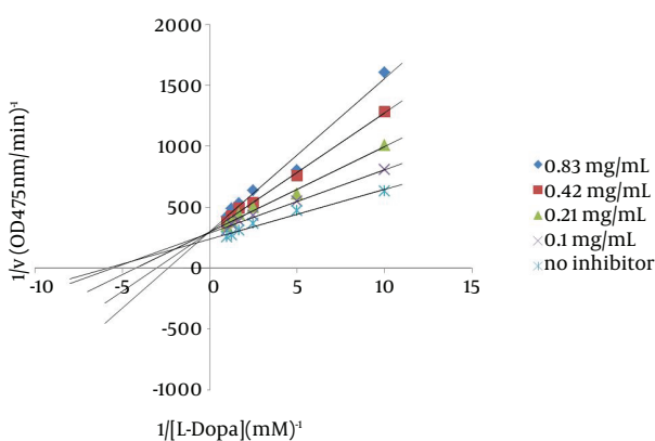
Figure 2. Lineweaver–Burk Plots of Mushroom Tyrosinase and L-Dopa With and Without P. alkekengi Different Concentrations
