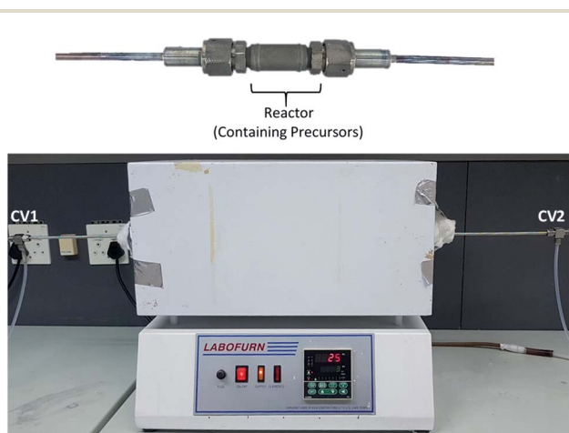
Fig. 1 Image of reactor and furnace setup, under argon atmosphere with a feed of 2 bar at room temperature, when heated to 350 °C. The manual control valves (CV1 and CV2) are open during purging (~1 h) and closed after initial purge. The quartz wool in the reactor outlet is to contain the precursors in the reactor and a beaker filled with water on the exit flow is placed while flowing Ar to monitor the gas flow and prevent air from entering the reactor.
