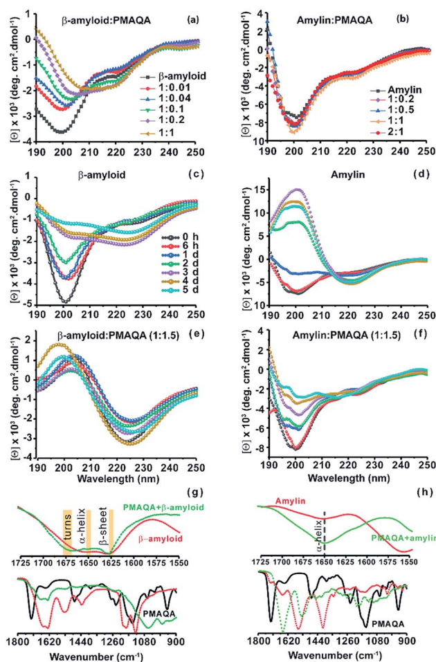
Fig. 2 Conformational analysis of \beta -amyloid-1-40 and amylin with and without PMAQA. Far-UV CD measurements showing the structural changes in 25 \mu\text{M} of \beta -amyloid-1-40 in 10 mM sodium phosphate, pH 7.4, (a) and in 25 \mu\text{M} of amylin in 30 mM sodium acetate, pH 5.5, (b) in the presence of PMAQA incubated for \sim 10 minutes at room temperature at the indicated peptide : PMAQA molar ratios (a and b). Time-lapsed structural changes in 25 \mu\text{M} \beta -amyloid-1-40 (c and e) and amylin (d and f) in the absence (c and d) and presence (e and f) of 1.5 molar equivalent PMAQA; time intervals used for results presented in c–f are indicated in (c). FT-IR spectra of \beta -amyloid-1-40 (g) and amylin (h) in the presence (green) and absence (red) of PMAQA obtained after 6 hours; peptide concentration and buffer conditions were as described for the samples used in CD measurements. Changes in the secondary structure of \beta -amyloid-1-40 are highlighted in yellow in the fingerprint regions ( 1550\text{--}1725\text{ cm}^{-1} ) (g, top).
