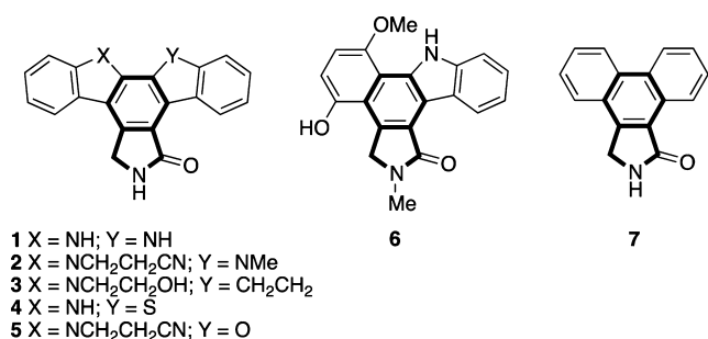
Figure 1. Polycyclic-fused isoindol-1-ones.
