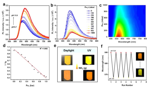
Fig. 5 (a) Emission spectra of LIFM-SHL-1 in aqueous dispersions with pH varying from 6.7 to 11.9; (b) photoluminescence spectra of LIFM-SHL-1 exposed to various fractions of ammonia and (c) 2D contours of the relationship between luminescence intensity and pressure of ammonia; (d) variation of the emission intensity with the pressure of ammonia; (e) response of the LIFM-SHL-1@PVDF membrane to \text{NH}_3 in daylight and photoluminescence color; (f) luminescence switching through alternately immersing LIFM-SHL-1@PVDF in pH 12.0 and pH 3.0 ammonia solutions.
