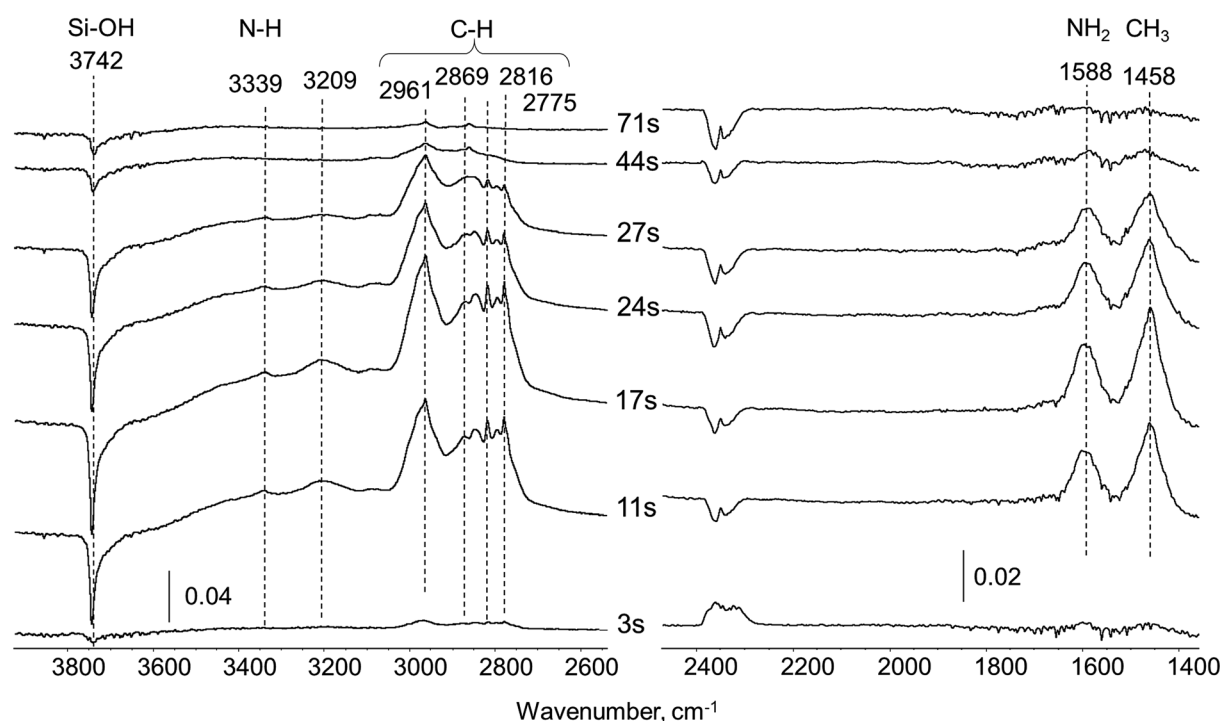
Fig. 2 Difference in situ FTIR spectra of silica carrier exposed to UDMH pulse (0.5 \mu l) in 20 ml min -1 He flow at 260 °C.
