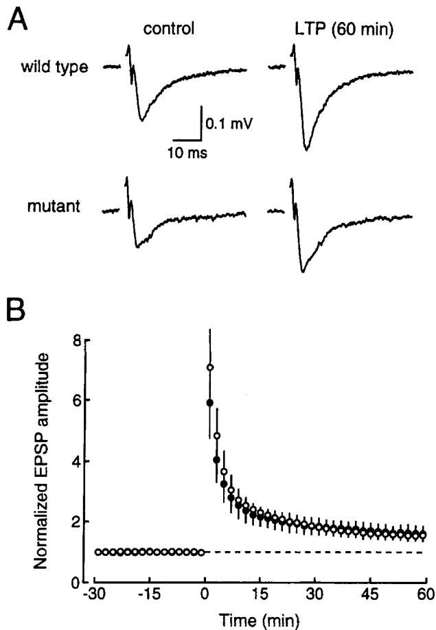
Figure 8. Mossy fiber LTP in area CA3 of hippocampal slices. (A) Typical recordings of mossy fiber fEPSP in the wild-type ( upper traces ) and mutant ( lower traces ) mouse before ( left ) and 60 min after ( right ) the induction of LTP. Each trace shows an average of 10 consecutive recordings. Stimulus artifacts are truncated. (B) Time course of mossy fiber LTP in wild-type (○; n = 10 slices) and mutant (●; n = 9) mice. Tetanic stimulation (see Materials and Methods) was applied at time 0. To exclude the possible contribution of inputs other than mossy fibers to LTP, 40 \mu M D-AP5 (D[-]-2-amino-5-phosphonopentanoic acid) was superfused for at least 7 min prior to the tetanic stimulation. Each point represents averaged fEPSP amplitude (mean \pm SD) normalized to base-line amplitude. All experiments were carried out without pre-knowledge of genotype.
