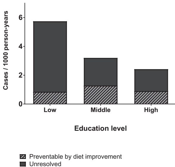
Fig. 2. Estimated proportion of cases that could be prevented if all participants adhered to a diet of a quality defined by quintile 5 of the LLDS. Based on confounder adjusted population attributable fractions, and incidence rates per educational level.
