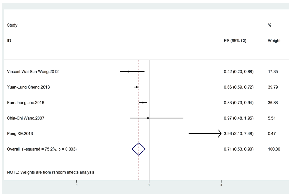
Figure 2: Forest plot showing the relationship between HBV infection and the risk of NAFLD. The horizontal axis is the X axis. The points represent the risk estimate of each individual study. Horizontal lines represent 95% confidence intervals; diamonds represent the summary risk estimate with 95% confidence interval. HBV, hepatitis B virus. NAFLD, nonalcoholic fatty liver disease. CI, confidence interval. ES, effect size.
