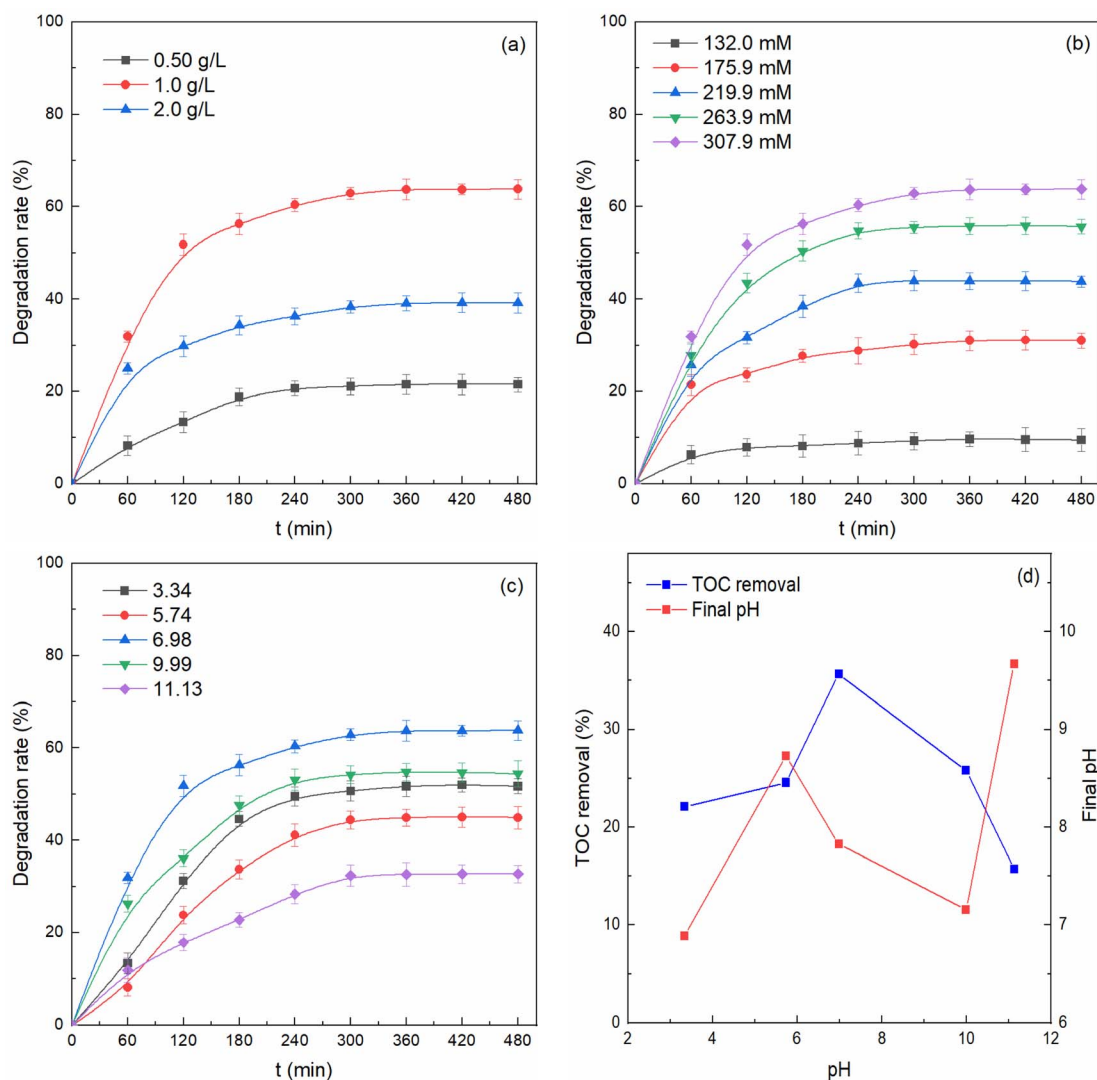
Fig. 6 Effect of reaction conditions on acetaminophen degradation through the heterogeneous Fenton reaction with Co/EMR: (a) catalyst dosage, (b) H 2 O 2 dosage and (c) initial solution pH; (d) TOC removal and the final pH after the reaction. With the exception of the evaluated parameter, the reaction conditions were as follows: [acetaminophen] 0 = 10 mg L -1 , [H 2 O 2 ] 0 = 307.9 mM, [Co/EMR] 0 = 1.0 g L -1 , initial pH = 6.98 (unadjusted), and T = 25 °C.
