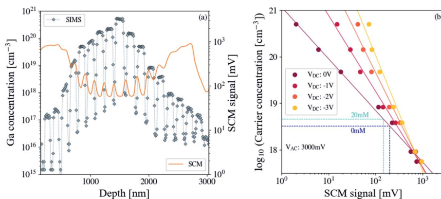
Fig. 6 Calibration curves for the SCM signal conversion into doping concentration. (a) SIMS is a chemical profiling technique while SCM is an electrical profiling technique. They are complementary techniques and superimposing their profile allows the conversion of the SCM signal into doping density. (b) Ga concentrations versus SCM data calibration curves for a set of DC biases ranging from 0 to -3 V: filled circles correspond to experimental values (minima of the SCM data and corresponding [Ga] in (a)) and solid lines are the linear fits of these experimental data.
