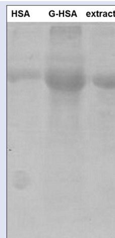
Figure 5: Electrophoretic pattern of native human serum albumin (lane on the left) and human serum albumin incubated for 8 week with 50 mM glucose without ( \mu\text{M} ) or with Perovskia atriplicifolia extract (lane on the right). The mobility retardation of G-human serum albumin is decreased in the presence of the extract
