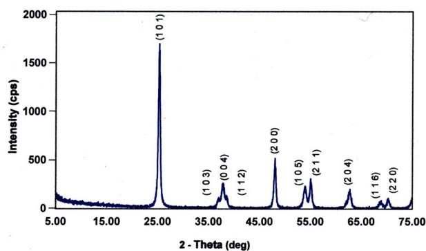
Fig. 2 The PXRD pattern for the sample with an average diameter \approx 12.69 \text{ nm} . The indexed peaks fit those in the JCPDS file #00-0634-0863 (ref. 120) for synthetic anatase titania.
