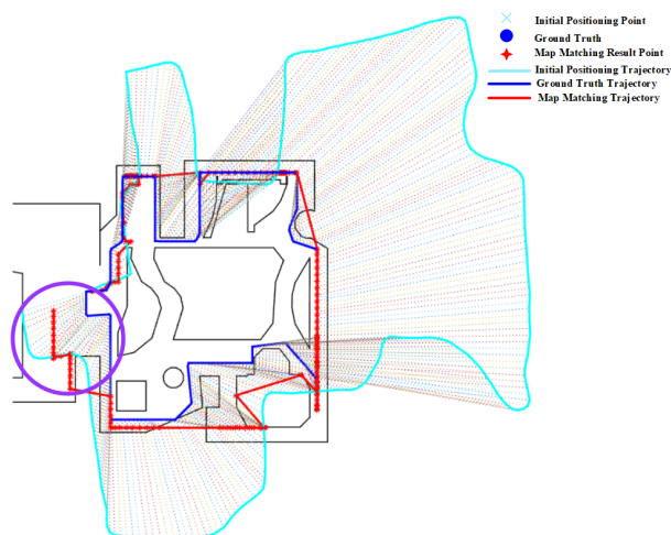
Figure 26. Positioning results of the geometric algorithm on Route 4 (Purple circle denotes the effect of Open Space).
