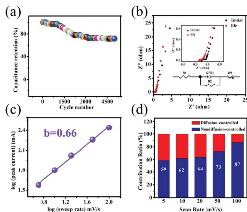
Fig. 4 (a) Cycling performances (at 10 \text{ mA cm}^{-2} ) of the Co(OH)F@NF electrode. (b) EIS spectrum of the Co(OH)F@NF electrode before and after 5000 cycles (inset is the corresponding equivalent circuit diagram). (c) Plots of \log(i) – \log(v) from 5 to 100 \text{ mV s}^{-1} for the Co(OH)F@NF electrode. (d) Ratio of the capacitive contribution from the non-diffusion-controlled process (blue) and diffusion-controlled process (red) to the charge storage of the Co(OH)F@NF electrode materials at different scan rates.
