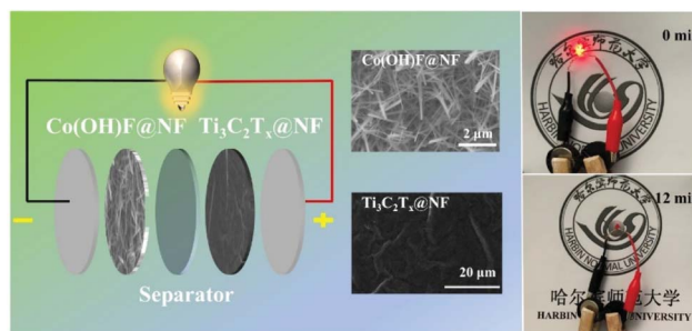
Fig. 6 Scheme of \text{Co}(\text{OH})\text{F@NF}/\text{Ti}_3\text{C}_2\text{T}_x\text{@NF} asymmetric supercapacitor and photographs of a LED powered by two coin cell asymmetric.
