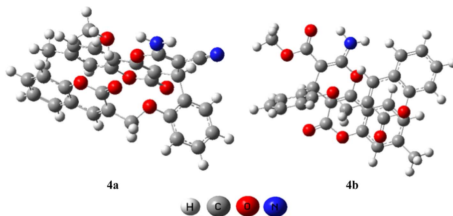
Fig. 5 The optimized structures of 4a and 4b .
