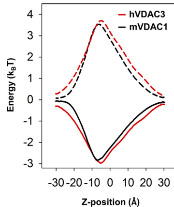
Figure S10. VDAC3 has a free energy profile similar to that of VDAC1. Ion transfer free energies for a chloride anion (solid lines) and a potassium cation (dashed lines) calculated for hVDAC3 (red) and mVDAC1 (black; see Materials and methods).
