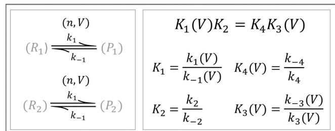
Figure 5. Reaction scheme with two charge-displacement pathways.
