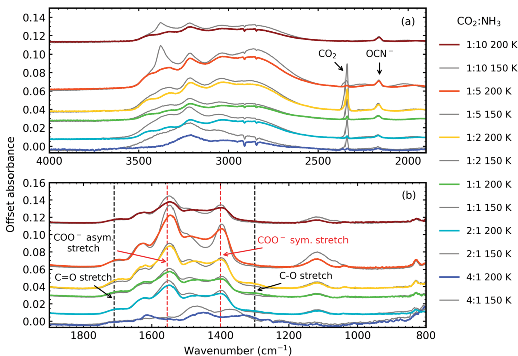
Fig. 5 Mid-IR spectra of CO 2 : NH 3 ices thermally processed to 150 K (grey traces) and 200 K (coloured traces) after irradiation with 1 keV electrons at 20 K. (a) 4000–2500 cm -1 including the N–H and O–H stretching region (4000–2500 cm -1 ) and CO 2 and OCN - features (b) 1900–800 cm -1 with dashed lines indicating the COO - asymmetric and symmetric stretches and C=O & C–O stretches. All spectra are normalised to a thickness of 400 nm and offset on the y-axis for clarity.
