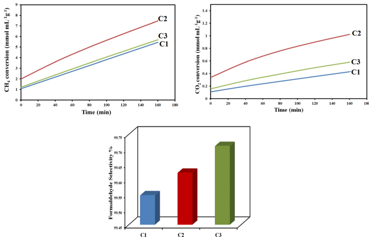
Fig. 7 Accumulative converted amounts of \text{CH}_4 and \text{CO}_2 with time and corresponding formaldehyde selectivity% using the Cu-Al LDH catalysts prepared at different MW power.
