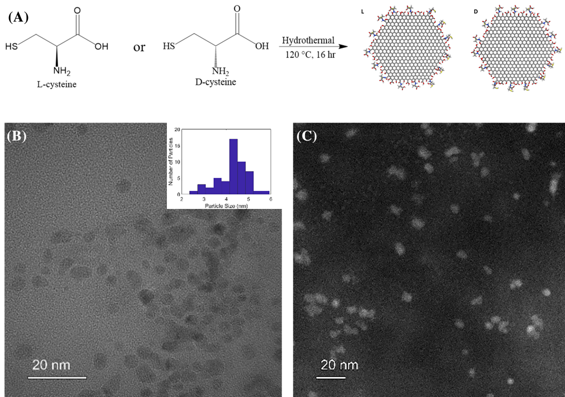
FIGURE 1 (A) Schematic of chiral CNP synthesis; the CNP cores are expected to contain both crystalline and noncrystalline areas (B) TEM of L -CNPs with histogram inset; and (C) STEM image of L -CNPs
