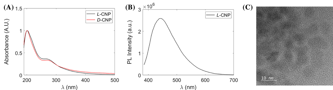
FIGURE 5 (A) UV-vis spectra; (B) emission spectrum; and (C) TEM image of L -CNPs following chiral separation
