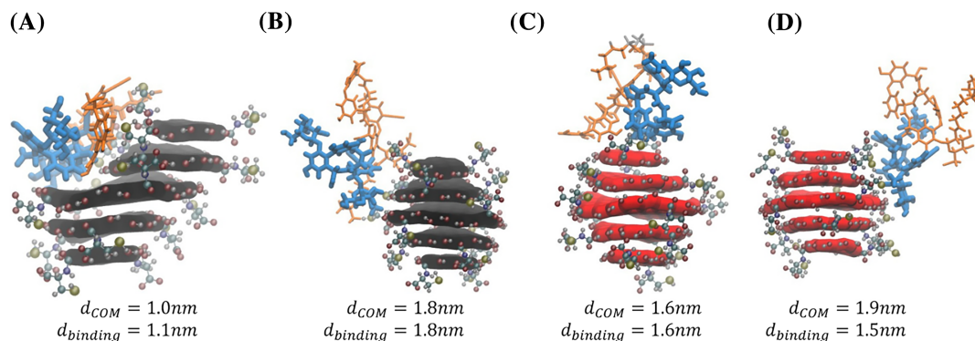
FIGURE 6 Chiral CNPs interacting with teicoplanin segments on the HPLC column. Teicoplanin (orange and blue), teicoplanin binding region (blue), D-CNP (red), and L-CNP (black)
