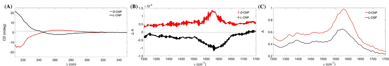
FIGURE 3 (A) CD spectra; (B) VCD spectra; and (C) IR spectra of chiral CNPs
