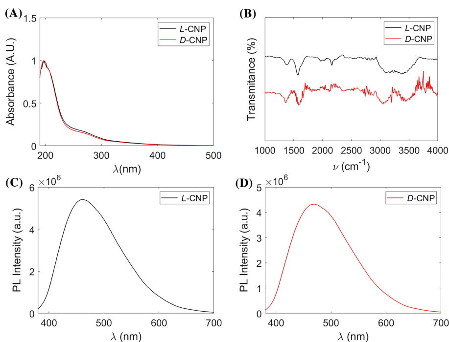
FIGURE 2 (A) UV-vis spectra of chiral CNPs; (B) FT-IR spectra of chiral CNPs; (C) PL spectrum of L-CNPs; and (D) PL spectrum of D-CNPs
