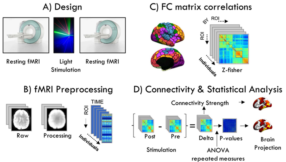
Figure 3. Workflow diagram. (A) The experimental design consisted of a repeated measures design where all the subjects underwent a resting fMRI session before and after receiving 1 min of light exposure to one of three wavelengths (green, blue, red) on three different days. (B) The fMRI analysis (see details in “Scanning protocol” section) yielded a time series for each individual. (C) The functional connectivity matrix for each subject was obtained after performing the Pearson correlation of the individual time series, and then we applied the Z-fisher transformation to perform the statistical analysis. The number of ROIs in the matrix correspond to the 100 ROI atlas used to extract the time series. (D) The connectivity analysis of the resting state networks was performed by computing the strength of connectivity within and between each network. To perform the statistical analysis, we first computed the difference between the FC post- and pre-stimulation yielding a delta matrix for each subject. These were used to perform the ANOVA repeated measures to find differences between the functional connections according to the kind of stimulation. This resulted in p value matrixes that were subsequently projected into the brain surface.
