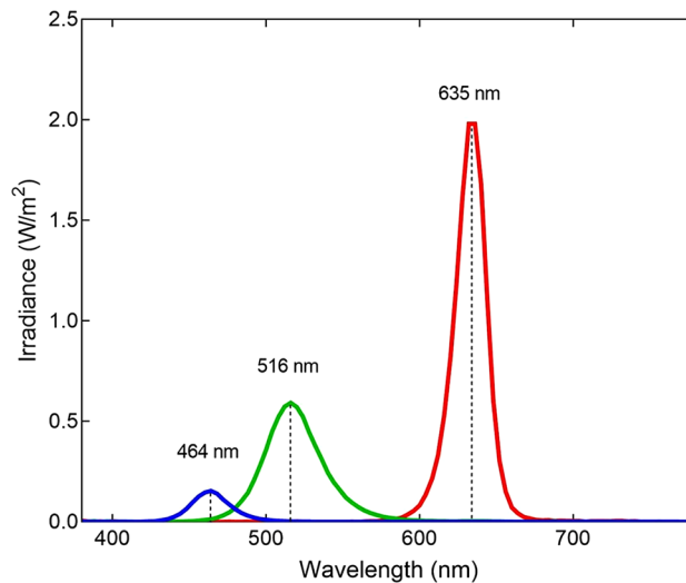
Figure 4. Spectral irradiance ( \text{W}/\text{m}^2 ) of the three monochromatic lights used in this study. Irradiance peaks are 464 nm (blue), 516 nm (green) and 635 nm (red).
