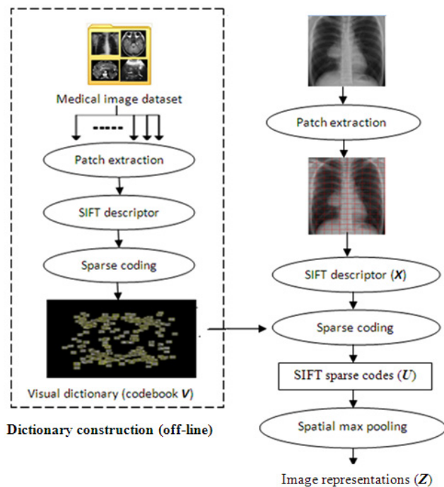
Fig. (8). Dictionary construction and image representations.
