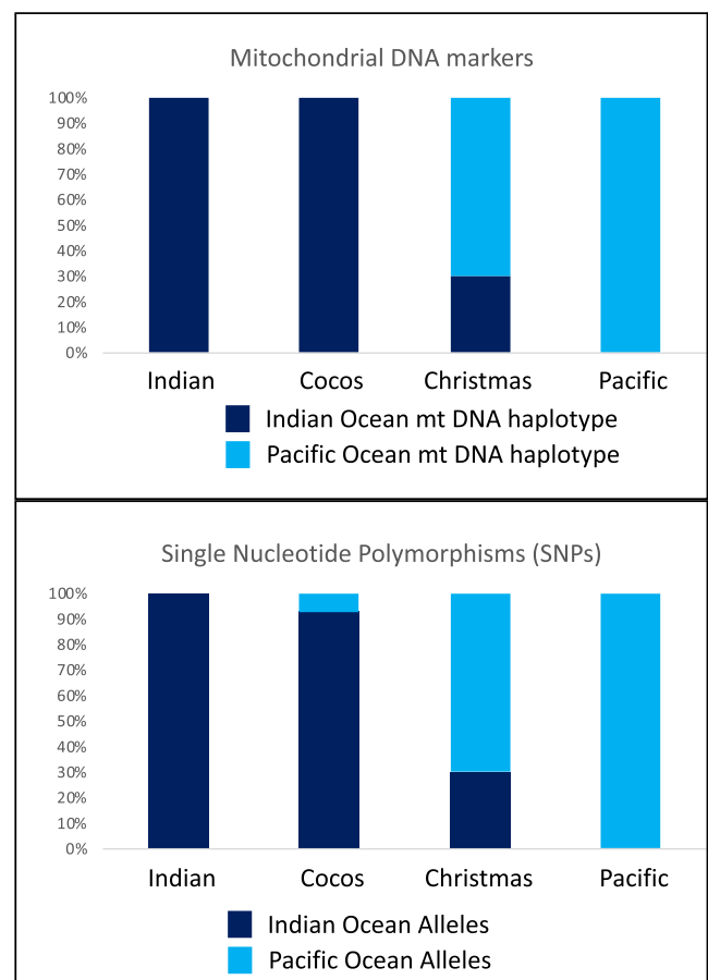
FIGURE 5 Top: Mitochondrial (mtDNA) haplotype frequency of the individuals from Cocos (Keeling) and Christmas Island. Bottom: Average allele frequencies of the 45 SNP loci that are fixed between the Indian and the Pacific lineage
