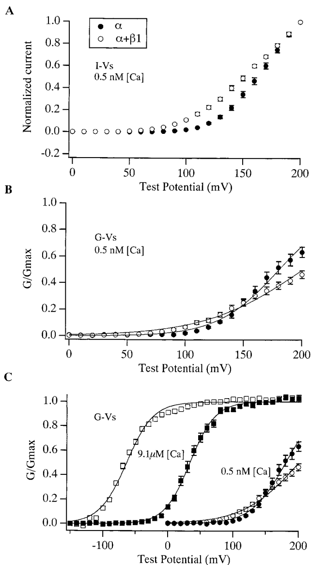
Figure 7. Effects of the \beta 1 subunit at subnanomolar [Ca^{2+}] . (A) Current-voltage curves for mSlo_{\alpha} ( \bullet , n = 11 ) and mSlo_{\alpha+\beta 1} ( \circ , n = 8 ) determined from patches superfused with a solution buffered to 0.5 \text{ nM } [Ca^{2+}] . Each current measurement was made at the end of a 50-ms voltage step to the indicated test voltage. Each curve has been normalized to their values at +200 \text{ mV} . (B) G-V relations were determined as described in the text from the same data as used to generate the I-V plots in A. Smooth curves represent Boltzmann fits. Parameters of the fits are: mSlo_{\alpha} V_{1/2} = 180 \text{ mV} , z = 0.98 , mSlo_{\alpha+\beta 1} V_{1/2} = 200 \text{ mV} , z = 0.61 . (C) In each experiment, data was acquired at both 9.1 \mu\text{M} (squares) and 0.5 \text{ nM } [Ca^{2+}] (circles). G-V plots for both concentrations are shown in C. In A–C, error bars indicate SEM.
