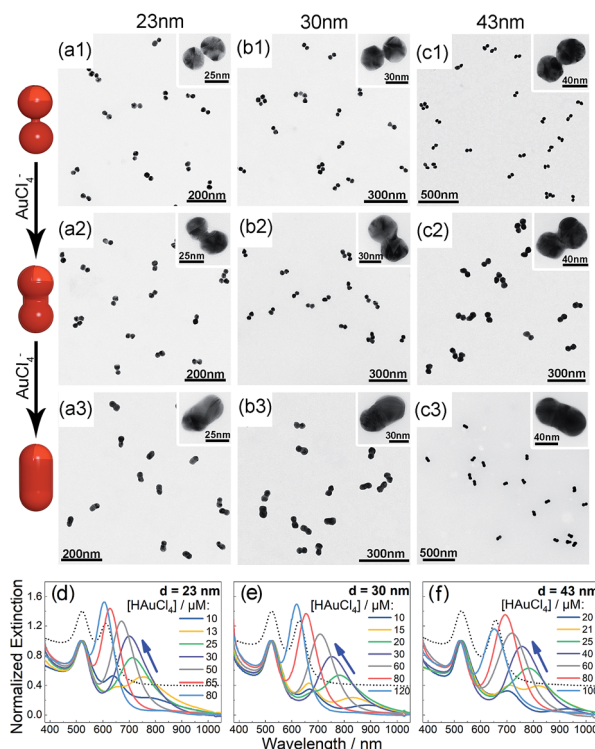
Fig. 1 (a–c) TEM images of the as-synthesized g-dimers with increased gold deposition (1–3) based on 23 (a), 30 (b), and 43 nm (c) AuNPs. Insets are magnified views of the CMNFs. (d–f) Extinction spectra of AuNP dimers after gold deposition to form tunable CTPs. Dotted curves indicate the BDP peaks (located at the right side of the 520 nm resonances) of unmodified dimers.
