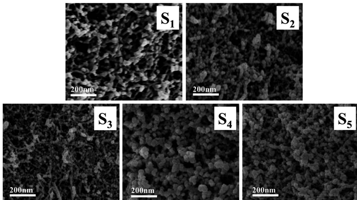
Fig. 7 SEM images of RF/Al 2 O 3 aerogels composites prepared with different RF/Al molar ratios (S 1 : RF/Al = 0.5, S 2 : RF/Al = 0.67, S 3 : RF/Al = 1.0, S 4 : RF/Al = 1.5, S 5 : RF/Al = 2.0).
