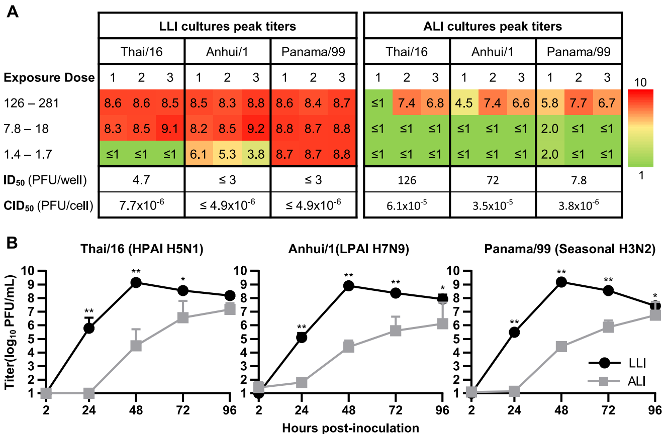
Fig. 5. Comparison of viral infectivity and replication between cells cultured at liquid-liquid (LLI) or air-liquid (ALI) interface. A) Peak viral titers detected in each well inoculated via the aerosol route, as described in the legend for Fig 3A. Exact exposure doses are listed in Table S2. Cells cultured at LLI and ALI were exposed concurrently and therefore have identical exposure doses. B) Replication curves from wells exposed to 116–260 PFU shown in panel A. Culture supernatants were collected at the indicated times p.i., and titers were determined by standard plaque assay to quantify infectious virus. The limit of detection was 10 PFU. Titters shown represent mean \pm standard deviation of three wells (two in the case of Thai/16). Two-way ANOVA showed that overall titer differences between cells cultured at LLI and ALI were statistically significant ( p < 0.05 ). For each virus, titers from LLI and ALI wells were compared at each individual timepoint ( p -values were adjusted for multiple comparisons using the Bonferroni correction): * indicates p < 0.05 , ** indicates p < 0.001 .
