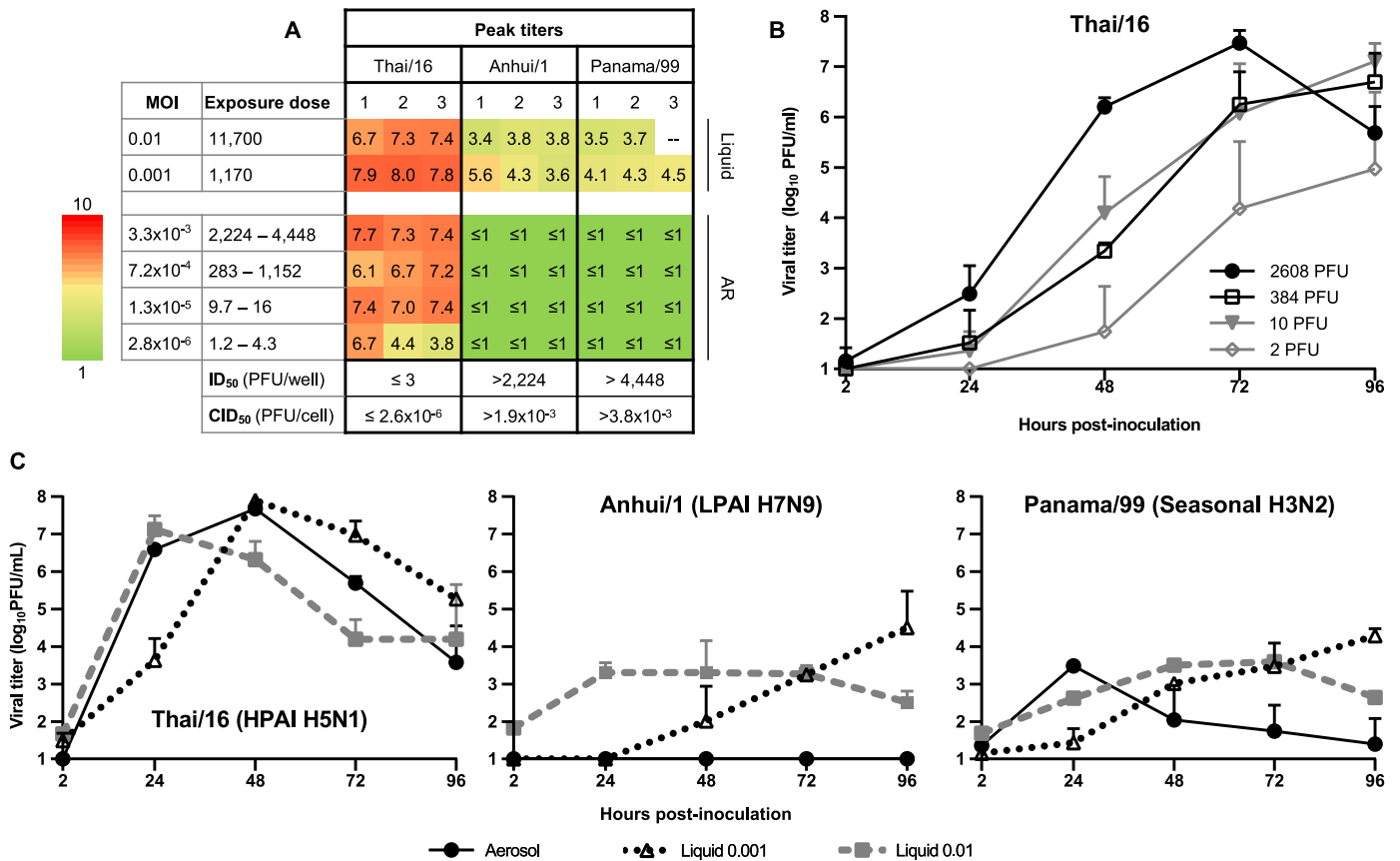
Fig. 4. Replication of influenza A viruses in primary human alveolar epithelial cells. A) Peak viral titers detected in each well inoculated via the aerosol route, as described in the legend for Fig. 3A. B) Replication curves for Thai/16 aerosol inoculations shown in panel A. Titers shown represent mean ± standard deviation of three wells. C) Comparison of replication kinetics subsequent to aerosol or liquid inoculation of human primary alveolar epithelial cells. Cells were infected by the aerosol route (solid black line), or by the traditional liquid route (dotted line) at an MOI of 0.01 (gray) or 0.001 (black). Aerosol MOIs were 0.002, 0.0006, and 0.002 for Thai/16, Anhui/1, and Panama/99 viruses, respectively. Culture supernatants were collected at the indicated times p.i., and titers were determined by standard plaque assay to quantify infectious virus. The limit of detection was 10 PFU. Mean ± SD from triplicate cultures (duplicate for Panama/99 liquid inoculum, 0.01 MOI) is shown.
