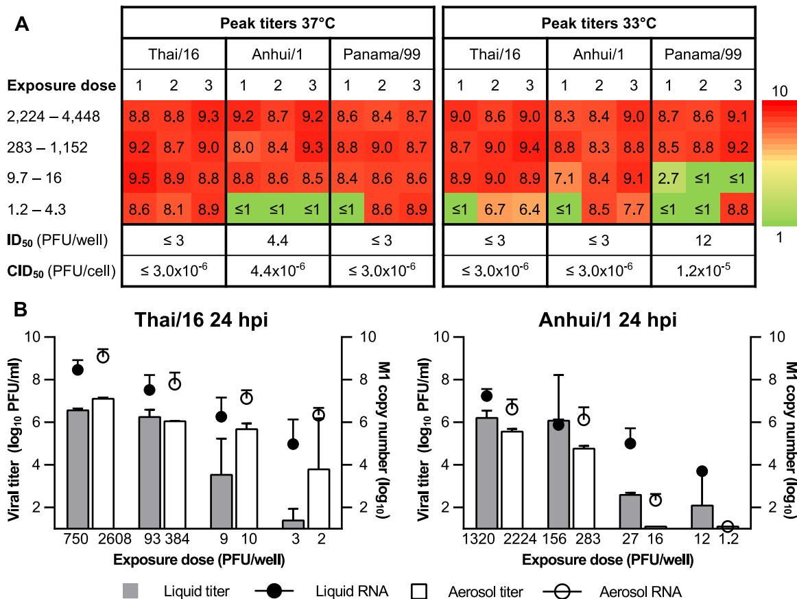
Fig. 3. Infection and replication in Calu-3 cells after aerosol exposure. A) Peak viral titers detected in each well inoculated via the aerosol route. Titers ( \log_{10} PFU/mL) are provided for each well that showed evidence of productive replication, defined as infectious virus detected at two sequential timepoints or at 96 h alone (full replication curves are shown in Fig. 2). Exposure dose (PFU) varied slightly between viruses and is therefore listed as a range. Exact exposure doses for each virus are listed in Table S1. Cells cultured at 33 and 37 °C were exposed concurrently. CID 50 indicates the 50% cellular infectious dose, or MOI required to achieve 50% infectivity, calculated by dividing ID 50 by the cell number. Limit of detection was 10 PFU. B) Comparison of viral supernatant titer (left Y axis) and M copy number (right Y axis) present in the cell monolayer between aerosol and liquid inoculation at 24 h p.i. Cells were cultured at 37 °C. Supernatants were collected immediately prior to lysis of the cell monolayer for RNA collection. Each parameter is expressed as mean \pm standard deviation of two independent wells. Limit of detection for M segment RNA was 10 copies.
