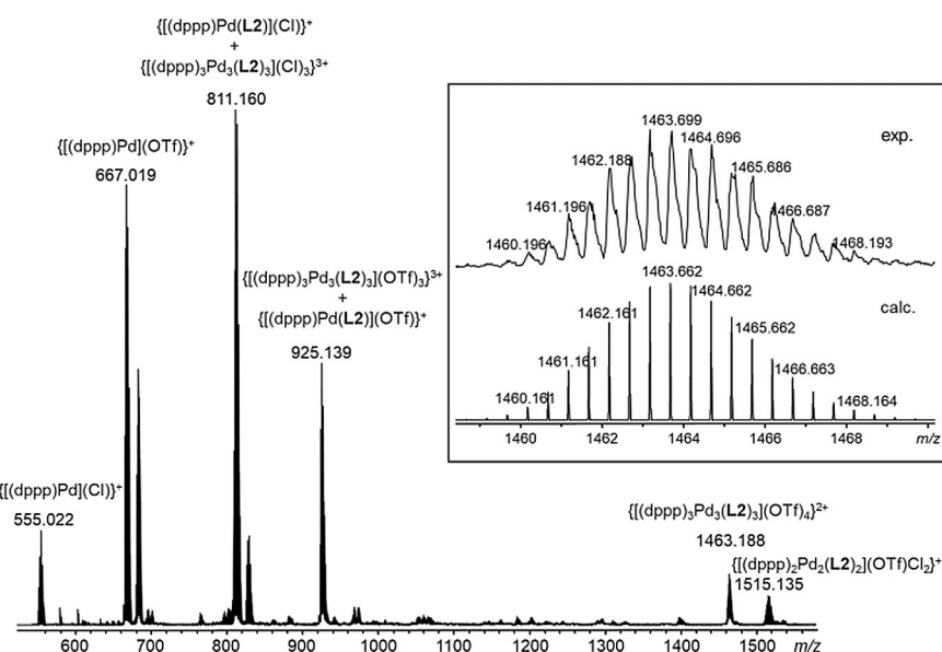
Figure 5. Positive ESI-MS spectrum of the 1:1 mixture of [(dppp)Pd(OTf)_2] and (rac)-L^{iso} showing signals of trinuclear 3:3 aggregates and their fragments. The inset shows the comparison of the experimentally determined isotope pattern of the \{[(dppp)_3Pd_3(L^{iso})_3](OTf)_4\}^{2+} ion and the calculated one.
