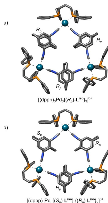
Figure 8. PBEh-3c/DCOSMO-RS( \text{NO}_2\text{CH}_3 ) optimized structures of the cationic units of trinuclear metallocsupramolecular triangles: a) the homochiral [(\text{dppp})_3\text{Pd}_3\{(\text{R}_p)\text{-L}^{\text{iso}}\}_3](\text{OTf})_6 and b) heterochiral [(\text{dppp})_3\text{Pd}_3\{(\text{R}_p)\text{-L}^{\text{iso}}\}_2\{(\text{S}_p)\text{-L}^{\text{iso}}\}](\text{OTf})_6 (hydrogen atoms are omitted, color scheme: carbon–grey, nitrogen–blue, phosphorous–orange, palladium–petrol, see Supporting Information for further details).
