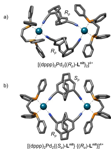
Figure 4. PBEh-3c/DCOSMO-RS( NO_2CH_3 ) optimized structures of the cationic units of dinuclear metallosupramolecular rhombs: a) homochiral [(dppp)_2Pd_2\{(R_p)-L^{niti}\}_2](OTf)_4 and b) heterochiral [(dppp)_2Pd_2\{(S_p)-L^{niti}\}\{(R_p)-L^{niti}\}_2](OTf)_4 (hydrogen atoms are omitted, color scheme: carbon–grey, nitrogen–blue, phosphorous–orange, palladium–petrol, see Supporting Information for further details).
