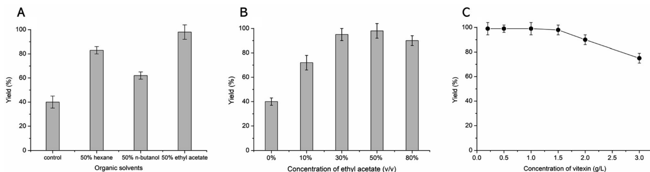
Fig. 2 Optimized bioconversion conditions for the glycosylation of vitexin. The effect of organic solvents (A), concentration of ethyl acetate (B) and concentration of substrate (C) on the vitexin glycosides yield.
