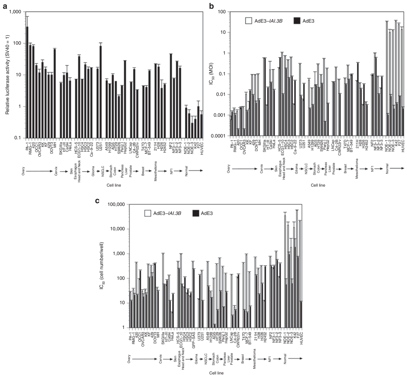
Figure 1 Tissue specificity of IAI.3B promoter, AdE3- IAI.3B and AdE3- IAI.3B -infected A549 carrier cells. (a) Transcriptional activity of the IAI.3B promoter in ovarian cancer, other cancer and normal cell lines. Bars, +SDs. (b) Cytotoxicity of AdE3- IAI.3B and AdE3 in ovarian cancer, other cancer and normal cell lines. Bars, +SDs. IC 50 , 50% inhibition rate of cell growth. (c) Cytotoxicity of A549 carrier cells infected with AdE3- IAI.3B and AdE3 in ovarian cancer, other cancer and normal cell lines. Bars, +SDs. IC 50 , 50% inhibition rate of cell growth.
