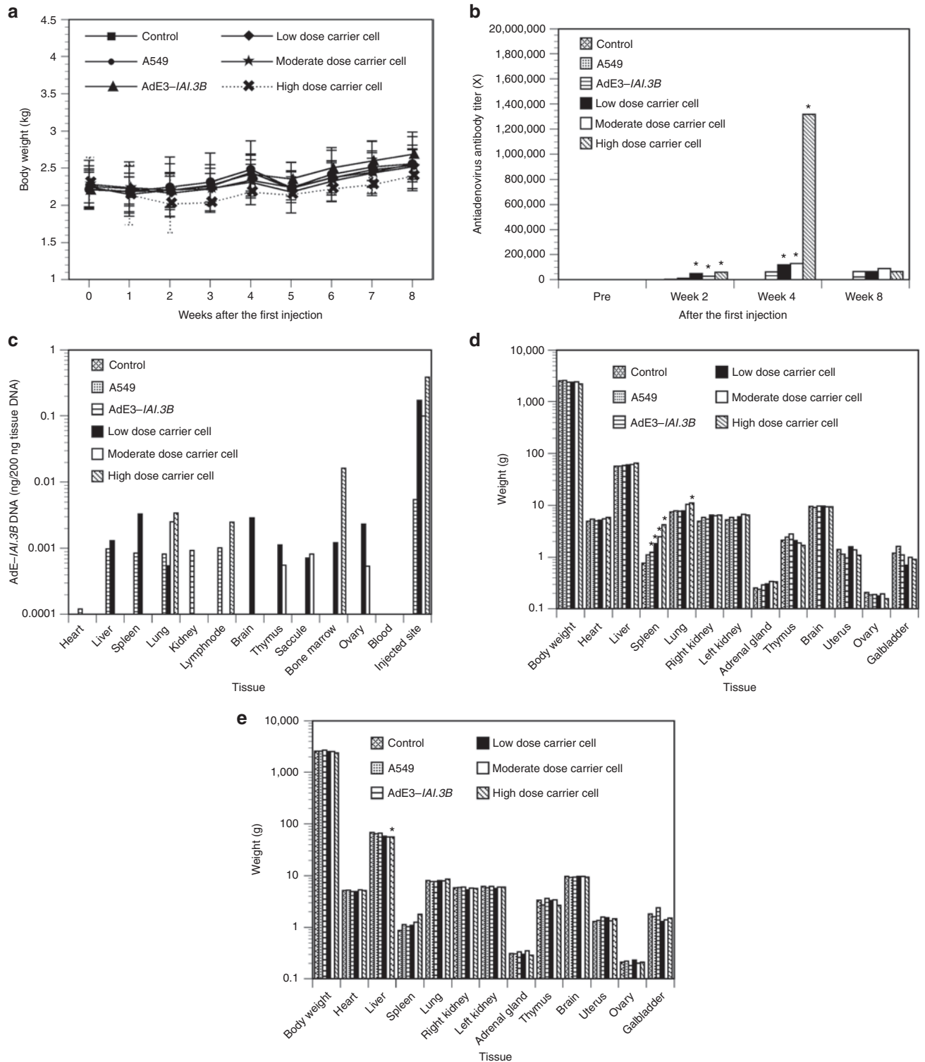
Figure 6 Chronic toxicity tests in rabbits. A549 cells, AdE3- IAI.3B , and low, medium and high dose of AdE3- IAI.3B -infected A549 carrier cells were subcutaneously administered to each rabbit on eight occasions over a 4 week periods. (a) Changes in body weight. (b) Changes in antiadenovirus antibody titers. (c) DNA content of AdE3- IAI.3B at 24 hours after the final injections with AdE3- IAI.3B -infected A549 carrier cells. (d) Weight of each organ at 24 hours after the final injections with AdE3- IAI.3B -infected A549 carrier cells (each dose without high dosage of carrier cells, n = 6 ; high dosage carrier cells, n = 2 ). (e) Weight of each organ at 4 weeks after the final injections with AdE3- IAI.3B -infected A549 carrier cells (each dose without high dose of carrier cells, n = 4 ; high dose carrier cells, n = 3 ). * P < 0.05 .
