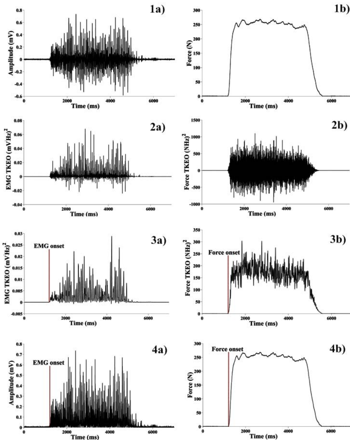
Figure 3 Process of EMG (a) and force (b) onset detection. 1a, b) Raw EMG and force signals. 2a, b) Teager Kaiser Energy Operator (TKEO) output for EMG and force signals. 3a, b) Full wave rectified and filtered TKEO outputs. Onset was detected at this stage using preset thresholds. 4a, b) Full-wave rectified EMG and raw force signals used to ascertain onset instances. The EMG signal and accompanying force curve depicted is from the right SpL of one of our participants during an extension effort.
