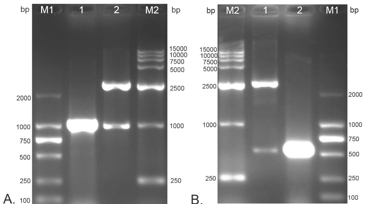
Figure 2 The construction of cloning plasmids were identified by colony PCR and restriction enzymes ( HindIII and XhoI ) digestion. M1, DNA marker-DL2000; M2, DNA marker-DL15000. A. Identification of cloning plasmid pMD18-T/ fgK . Lane 1, product of the colony PCR; Lane 2, two fragments after digestion of the recombinant DNA with restriction enzymes HindIII and XhoI . B. Identification of cloning plasmid pMD18-T/ tgK . Lane 1, two fragments after digestion of the recombinant DNA with restriction enzymes HindIII and XhoI ; Lane 2, product of the colony PCR.
